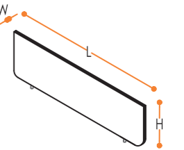
MASA ÜZERİ YAN PANEL/KUMAŞ LIGHT PANEL FOR EXTENSION TABLE/FABRIC
