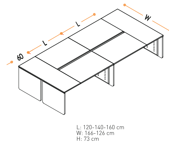
YAN İLAVELİ DÖRTLÜ GRUP MASALAR ORTAK AYAK İLE / WORKSTATION FOR FOUR
