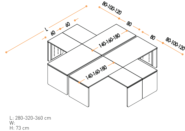
DÖRTLÜ GRUP MASALAR / WORKSTATION FOR FOUR
