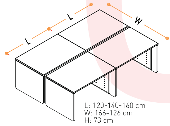
DÖRTLÜ GRUP MASALAR ORTAK AYAK İLE / WORKSTATION FOR FOUR WITH MIDDLE LEG
