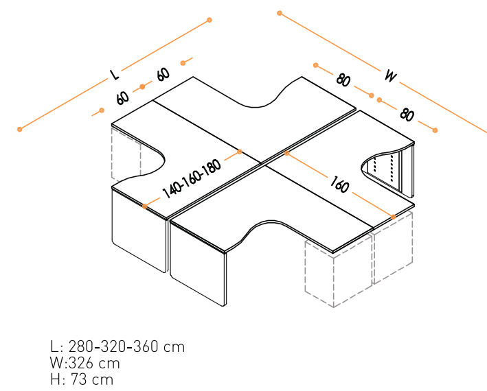
DÖRTLÜ GRUP G MASALAR / WORKSTATION FOR FOUR - G TABLE
